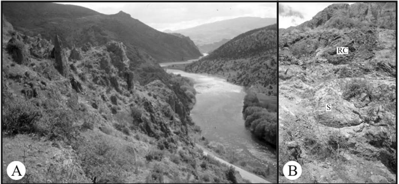
Fig. 3 - A. General view of the Dağkumlu Mélange within the Sakarya Valley; B. Tectonic relationship between the radiolarian chert blocks (RC) and serpentinites (S).
