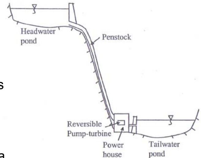
Figure 12.13 A typical pumped-storage plant.
