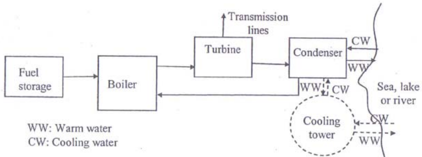
Figure 12.1 Operational scheme of a thermal power plant.
