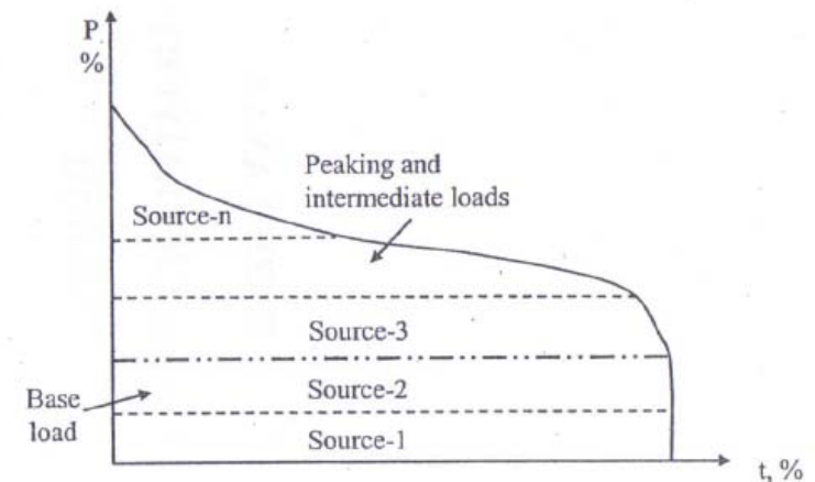
Figure 12.7 A typical load duration curve.
