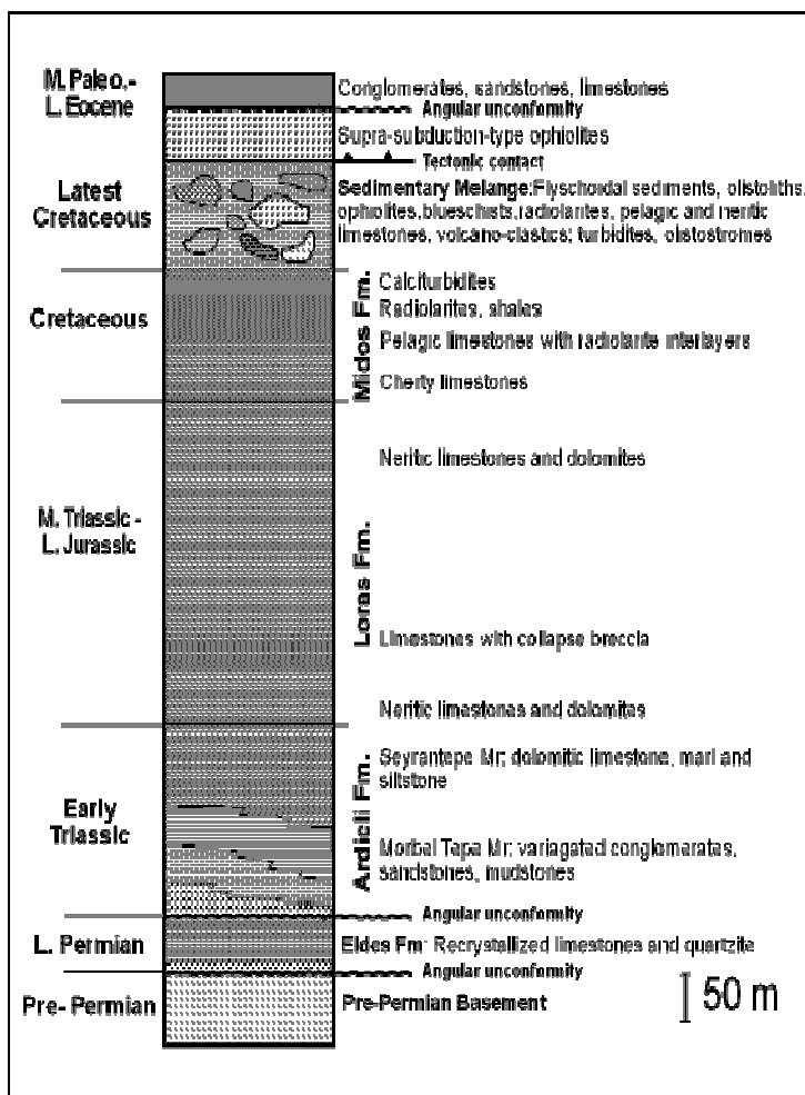
Figure 2- Generalized stratigraphy of the Tauride-Anatolide margin sediments in the Kütahya-Bolkardağ Belt
