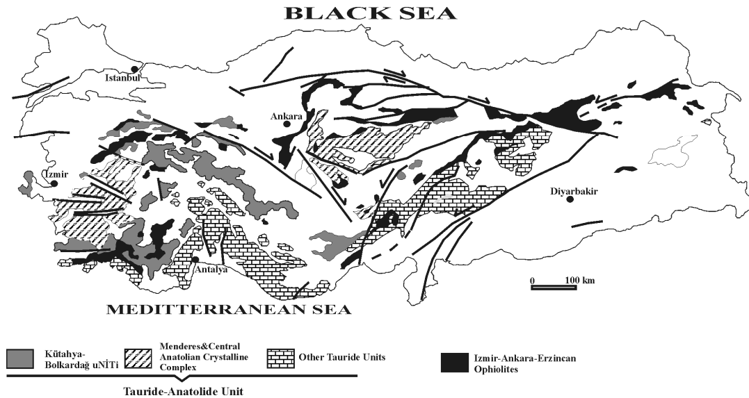
Figure 1- Location and distribution of the Kütahya-Bolkardağ Belt within the Tauride-Anatolide Terrane.
